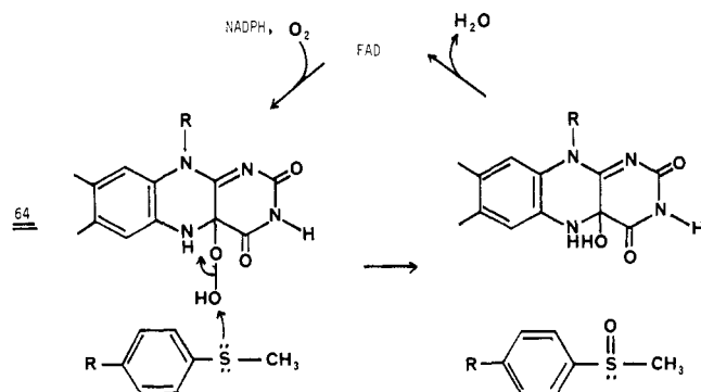
Figure 6. Proposed route for S-oxidation by flavin-dependent monooxygenases.
