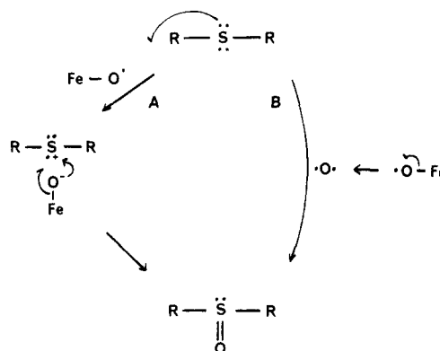
Figure 5. One- and two-electron routes for S-oxidation by cytochrome P-450 monooxygenases.
